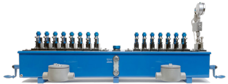
15 feed rear auxiliary shaft driven pump to point system with dual electric heaters, and shaft rotation alarm
